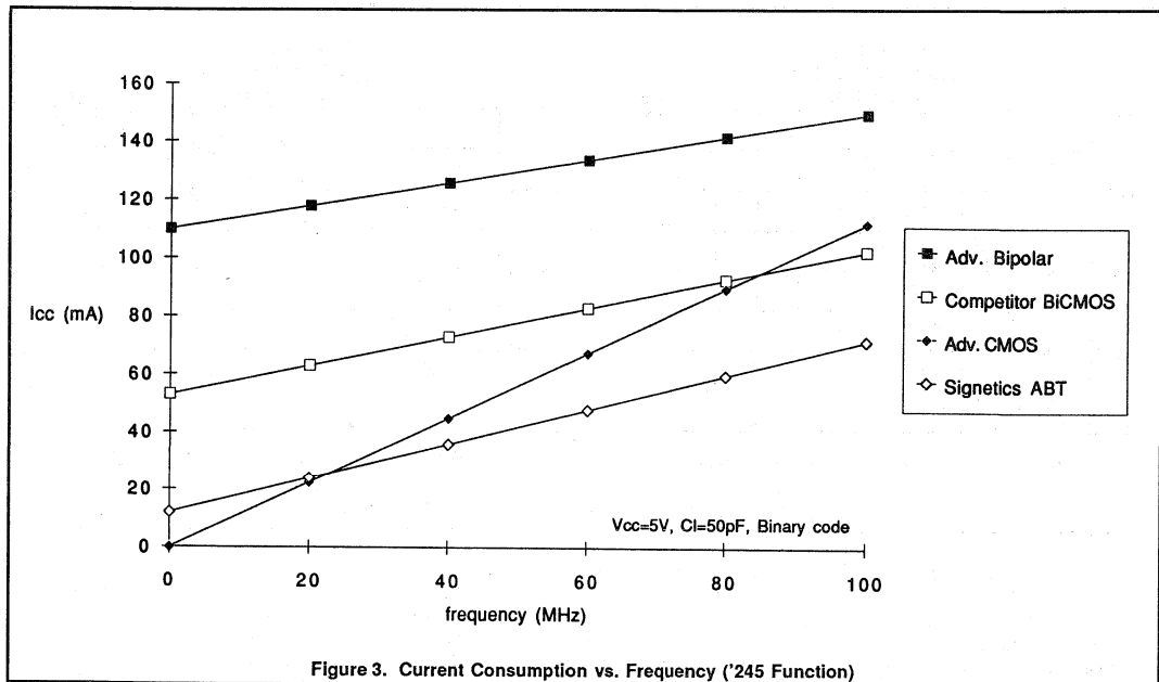
Figure 3. Current Consumption vs. Frequency ('245 Function)
