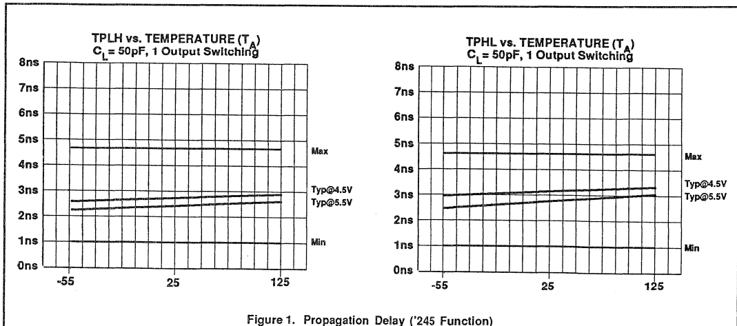
Figure 1. Propagation Delay ('245 Function)
