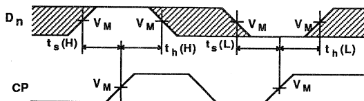
Waveform 3. Data Setup And Hold Times
